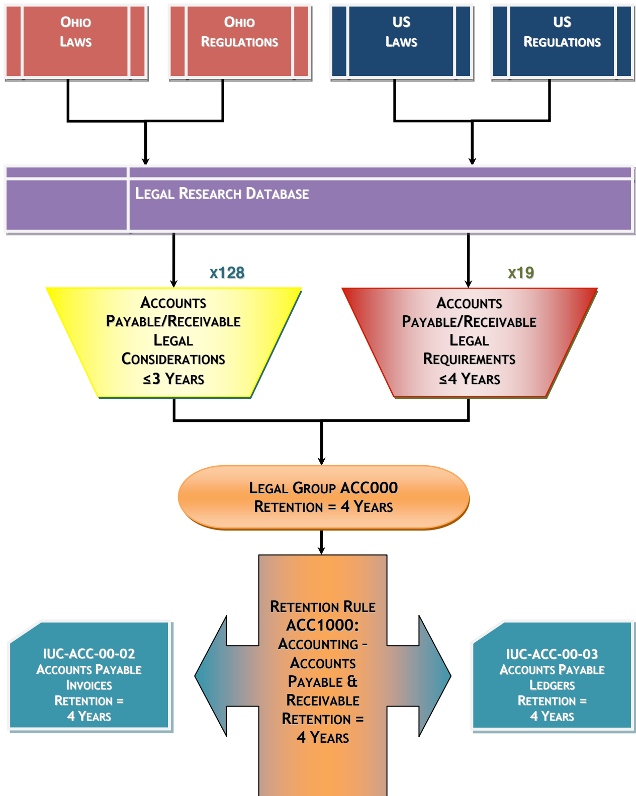
Figure1: Skupsky Model
